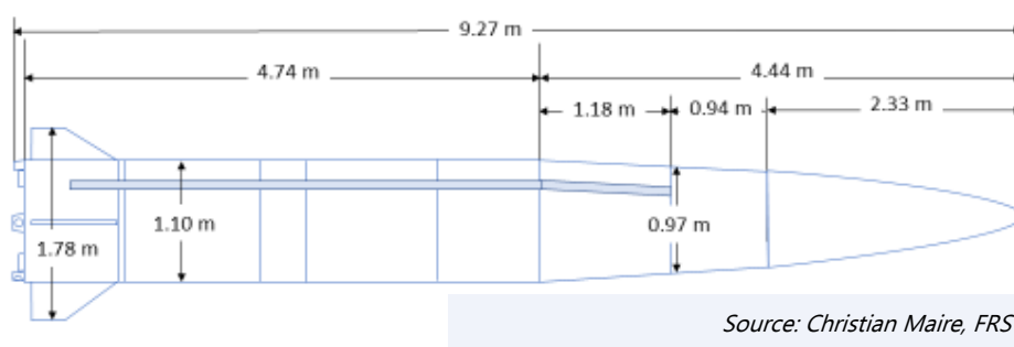
Figure 31. KN-23 and KN-23A upper sections
